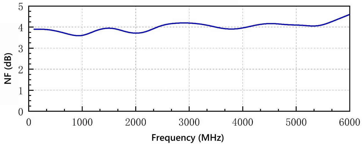
NF VS Frequency
